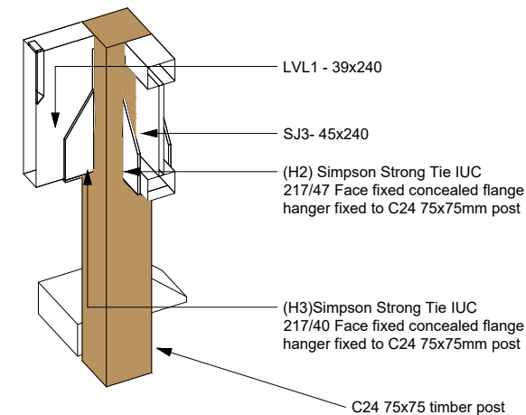
2 Post Head Connection
